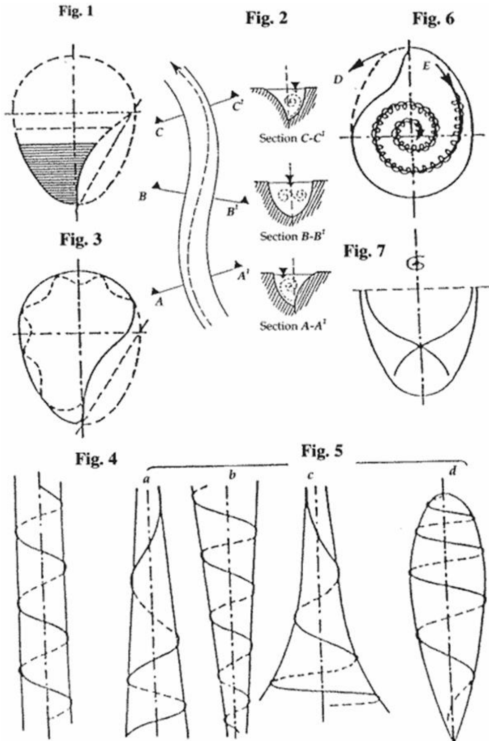
Fig. 18: Double spiral pipe diagram – multiple patents
