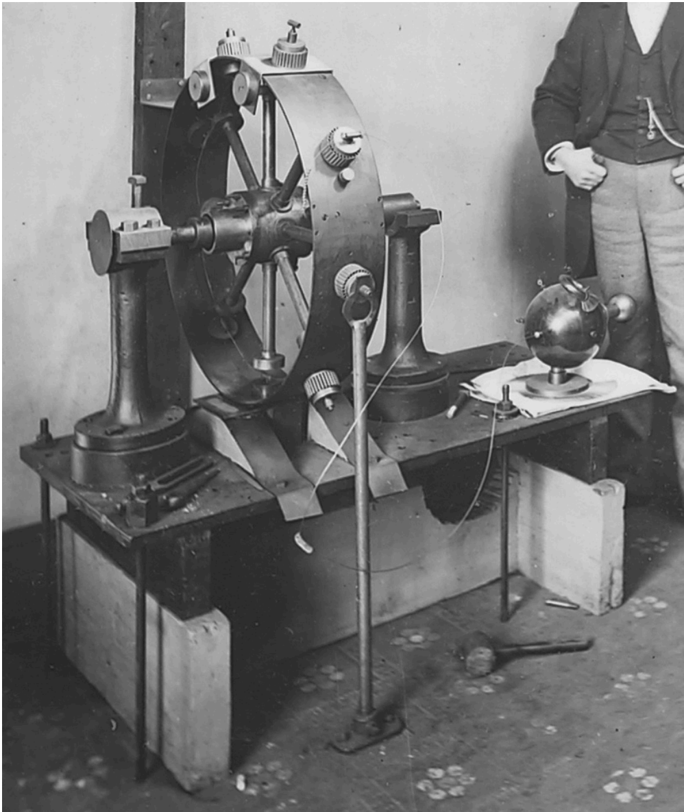
The Vibrodyne and Sympathetic Transmitter
