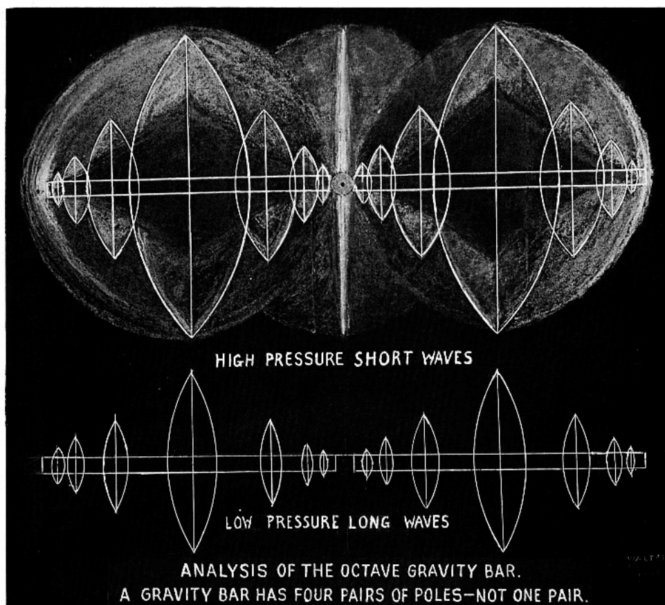
Figure 17.03 - Analysis of the Octave Gravity Bar. (courtesy University of Science and Philosophy )
