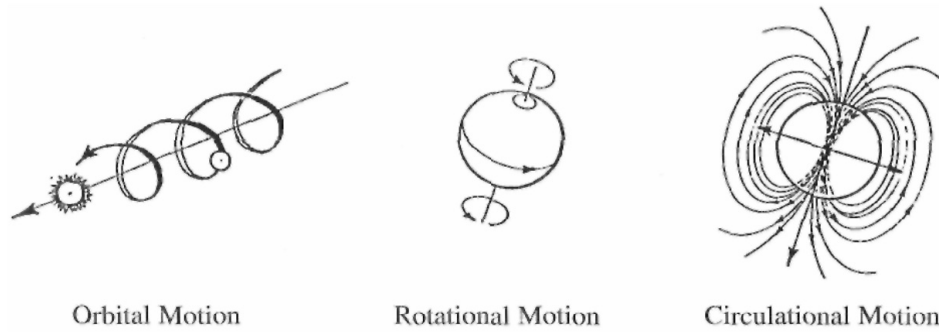
Fig. 9: The natural tripartite motion of the Earth
