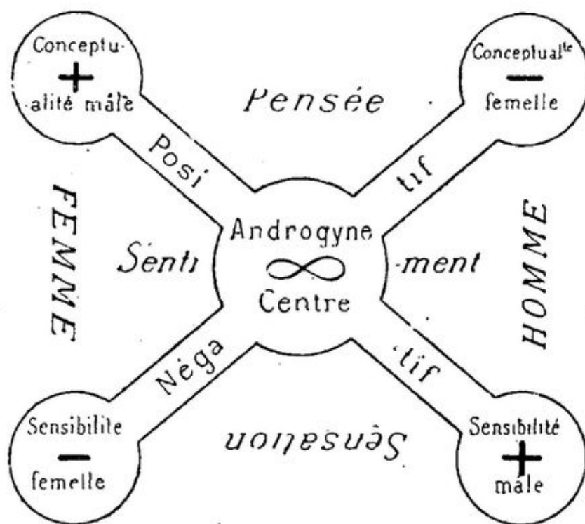
Four Fundamental Phases of Polarity
