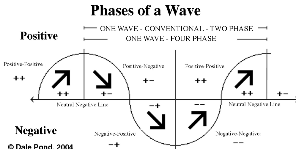
Figure 8.11 - Four Fundamental Phases of a Wave
