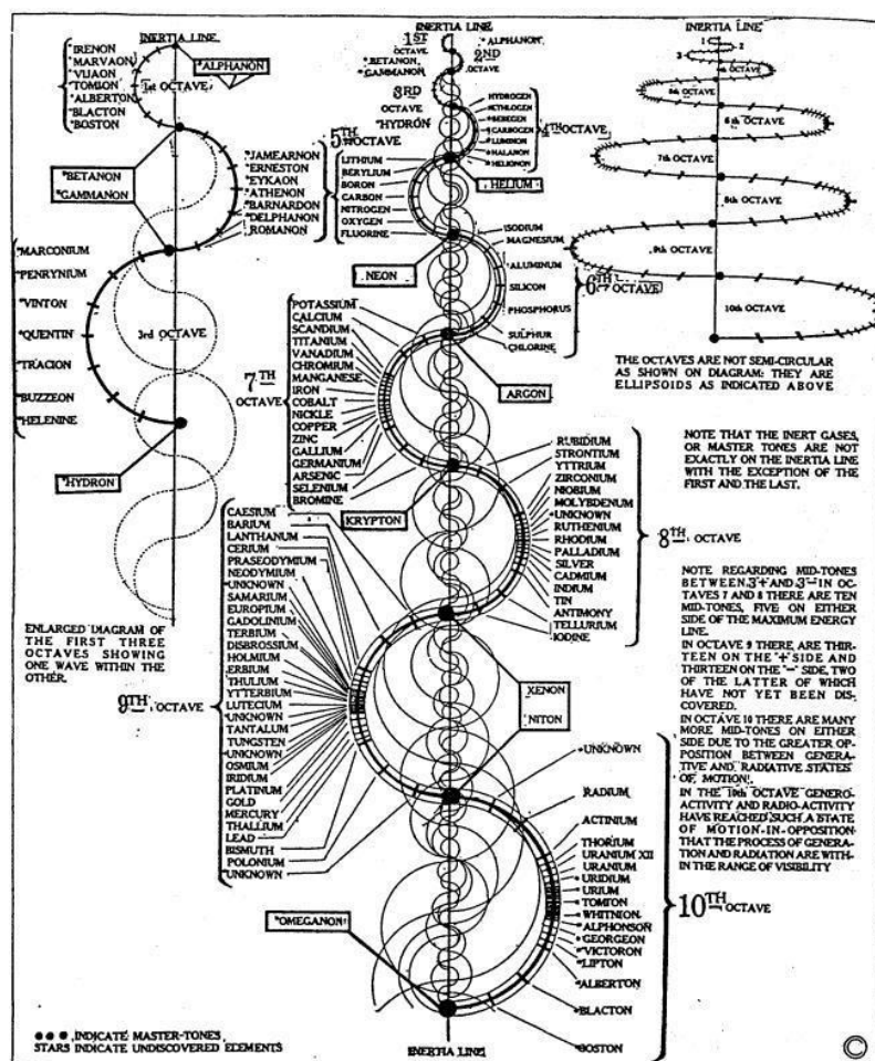
Figure 7B.08 - Russells Periodic Chart of the Elements
