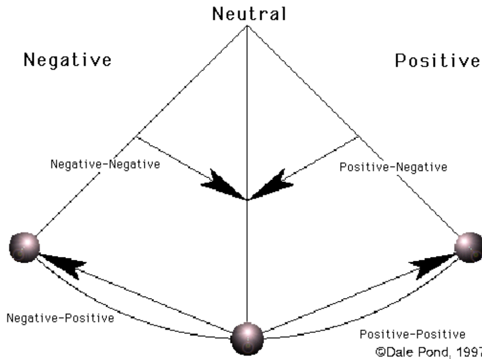
Figure 2.7 - Swinging Pendulum showing equal but opposed Polar States
