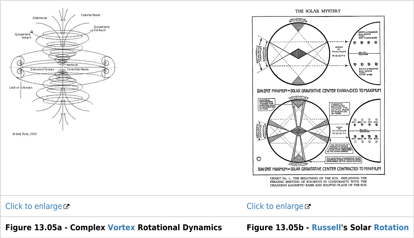
Figure 13.05a - Complex Vortex Rotational Dynamics
