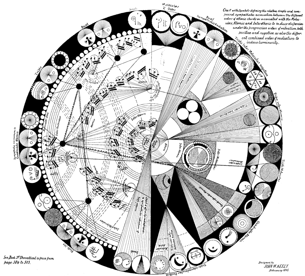
Figure 1.10 - Keely's Vibratory Relations of Multi-Level Matter (showing the nested levels of quantum entity relations)
