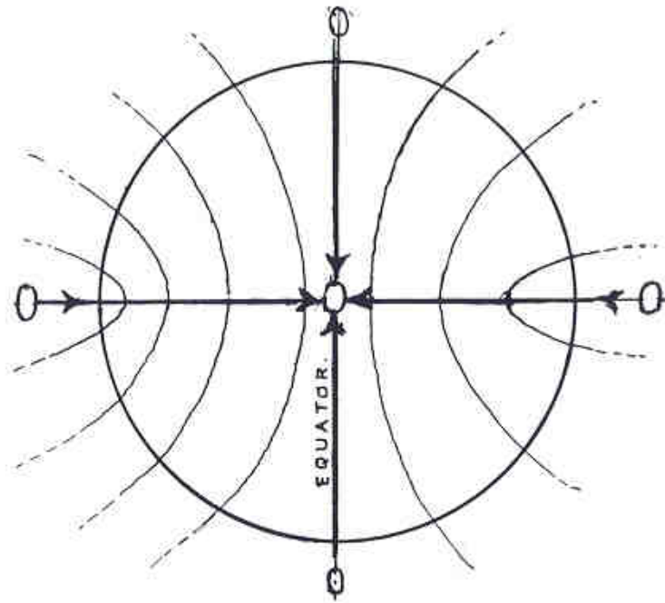
FIG. 61. Illustrating the bilateral nature of matter and the seeming curvature of gravity.
