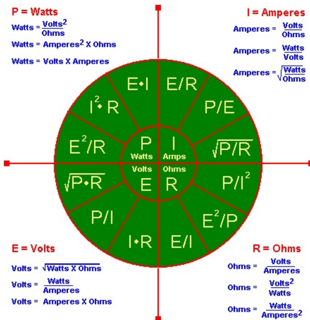
Current, Power, Resistance and Work Relationships
