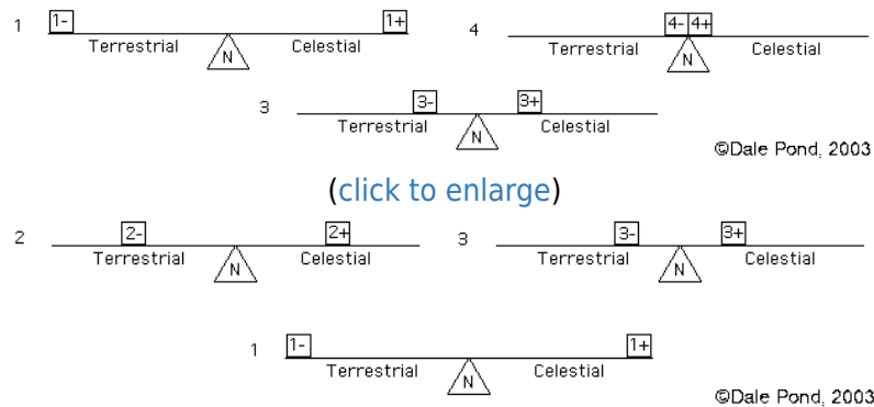
Figure 13.16 - Compound Equilibrium States
